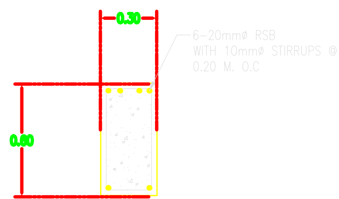
DETAILS @ 'A'
