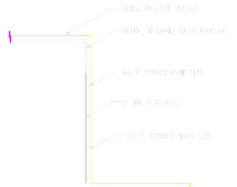
DIVING POOL DETAIL OF END WALL
