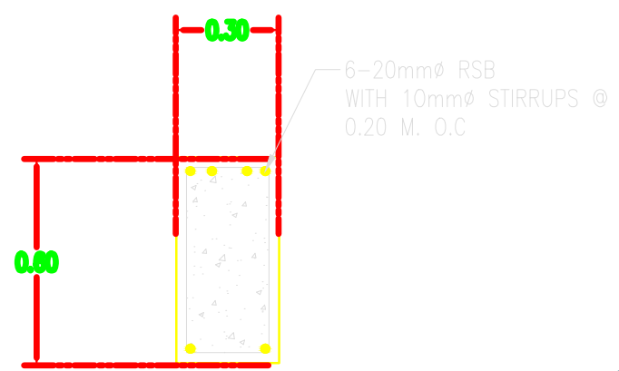
DETAILS @ 'A'
