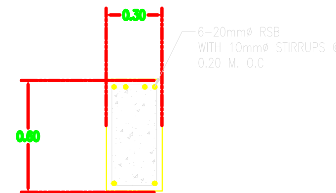
DETAILS @ 'A'
