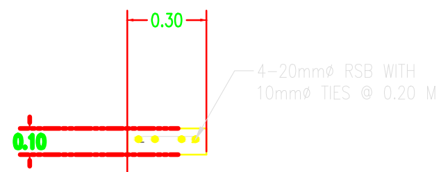
DETAILS @ 'B'
