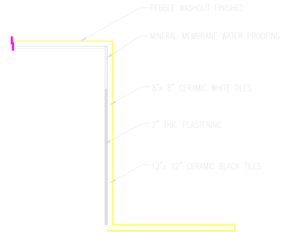
DIVING POOL DETAIL OF END WALL
