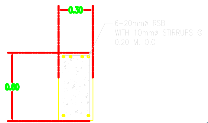
DETAILS @ 'A'
