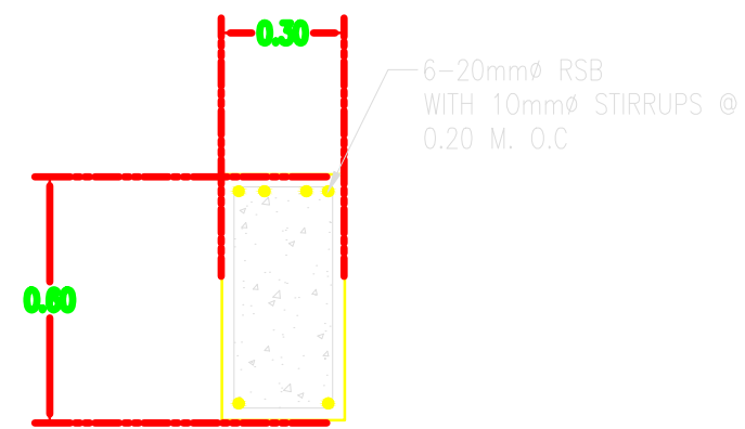
DETAILS @ 'A'
