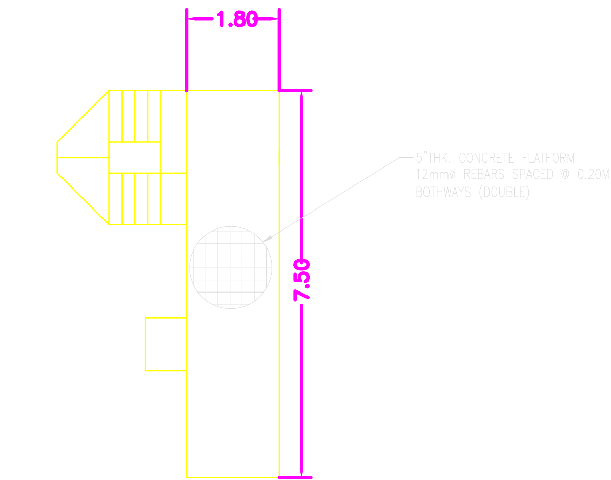
FIRST LEVEL @ 5.00M
