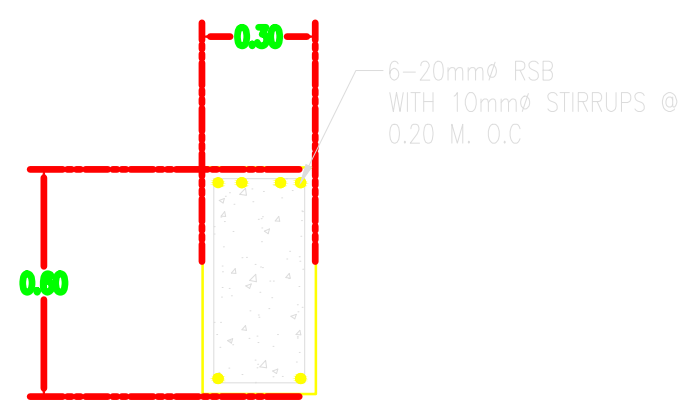
DETAILS @ 'A'
