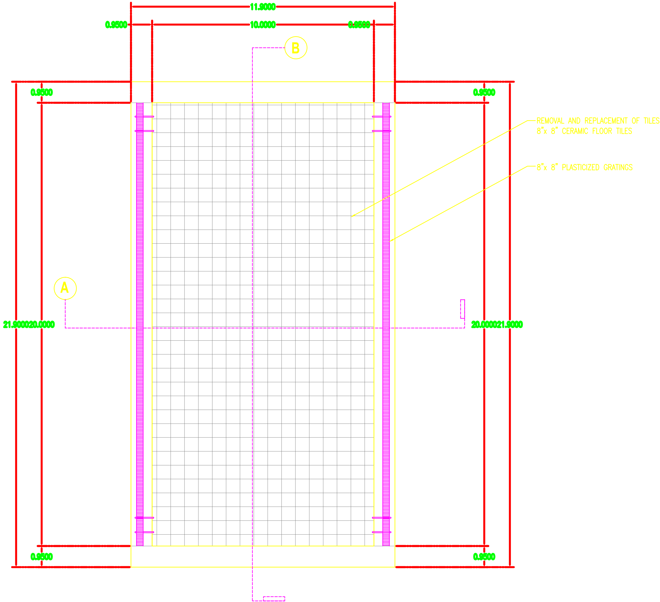
PROPOSED WARM-UP POOL PLAN SCALE 1 : 100 MTS.
