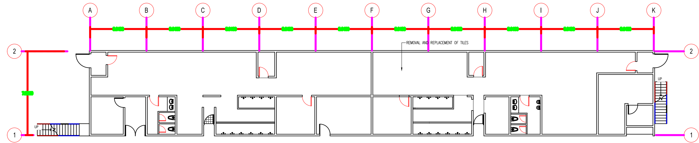
EXISTING GROUND FLOOR PLAN SCALE 1 : 100 MTS.
