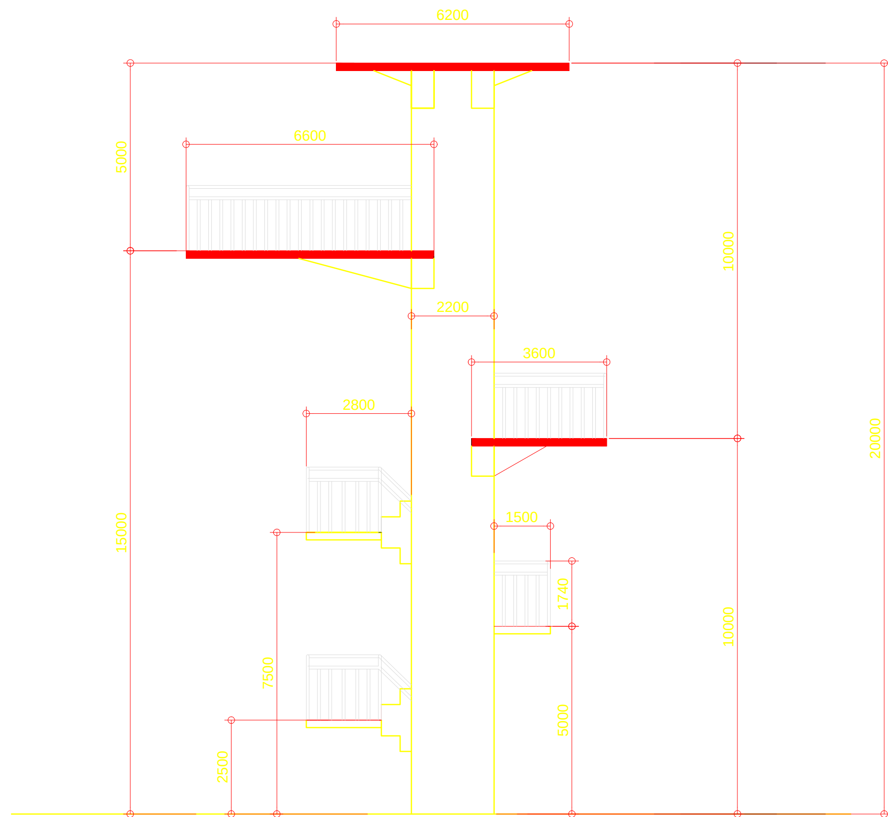
DIVING PLATFORM FRONT ELEVATION SCALE 1:200 MTS.
